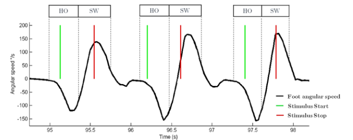
Figure 2 Example of stimulation triggering based on Equ 2 from an experimental record. In green and red are respectively the start and stop actual stimulation events triggered by the non-stationary period detection algorithm. Heel off (HO) and swing (SW) phases were manually added to the figure from literature for reference.
